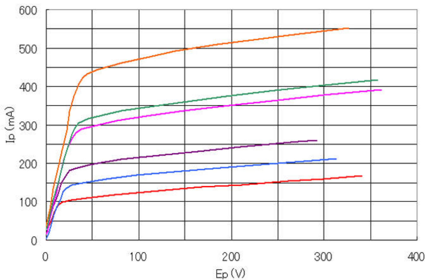
6HJ5 Ep-Ip Curve E_g=0V
