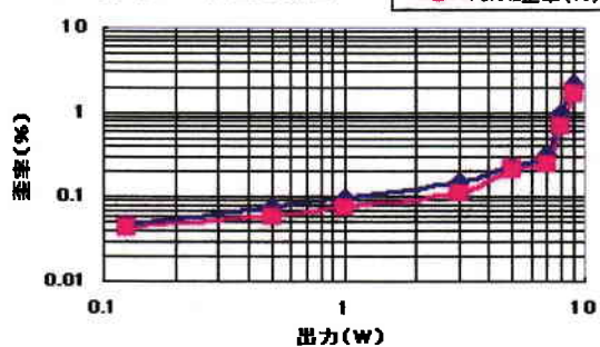
CasComp6V6pp歪率特性
