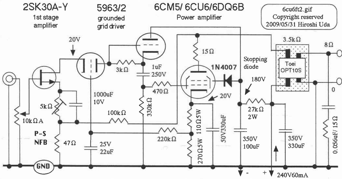
Fig: Schematic of J-FET~triode cascade SRPP driven 6CU6 etc. single amp
