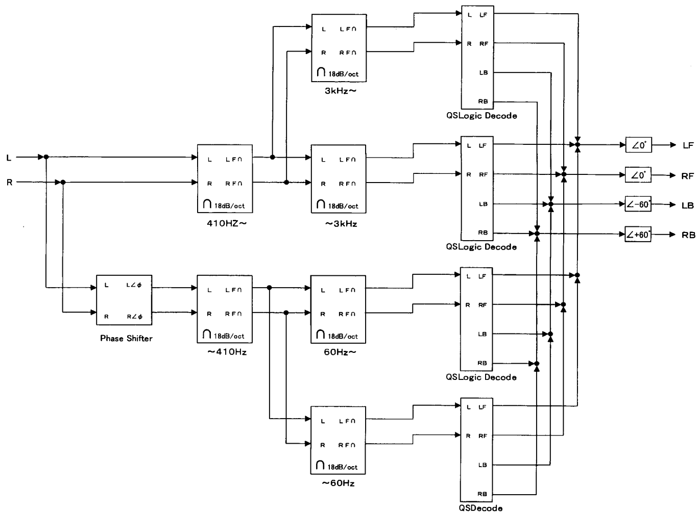
QS Three Band Full Logic Decoder Block Diagram
