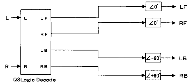
QS One Band Full Logic Decoder Block Diagram
