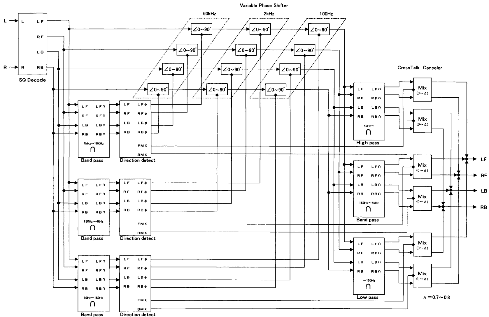
SQ Three Band Full Logic Decoder Block Diagram
